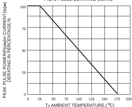
FIG. 2-PULSE DERATING CURVE
