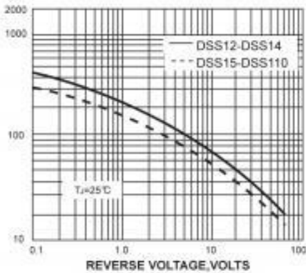
FIG. 5-TYPICAL JUNCTION CAPACITANCE
